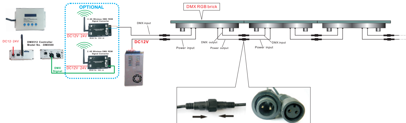
Wiring Diagram (4)
