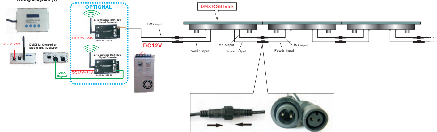
Wiring Diagram (4)
