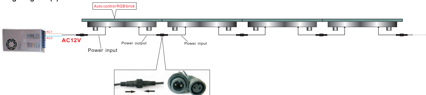
Wiring Diagram (2)
