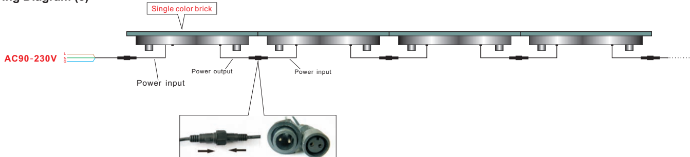
Wiring Diagram (3)
