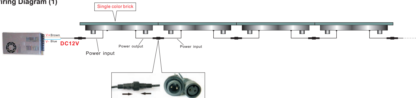
Wiring Diagram (1)
